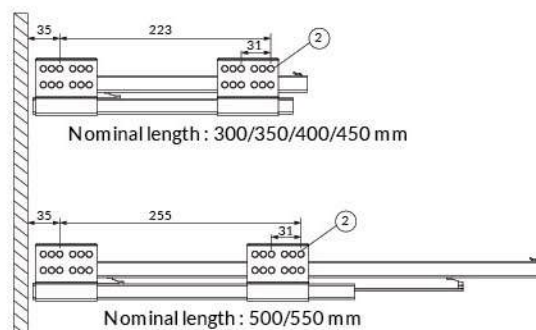
Product Breakdown Drawing
