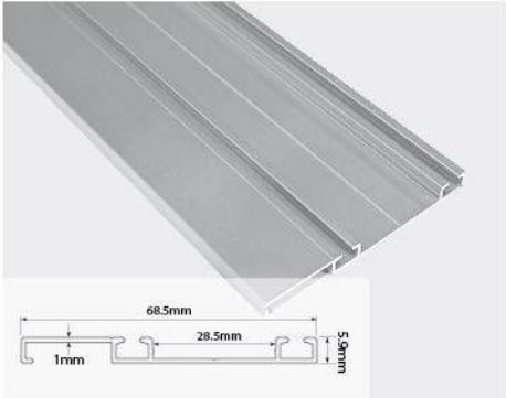
WSP-12 Sliding Bottom Profile
