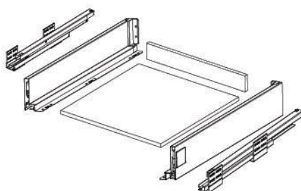
Product Breakdown Drawing
