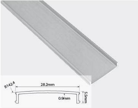
WSP-12C Bottom Cover Profile
